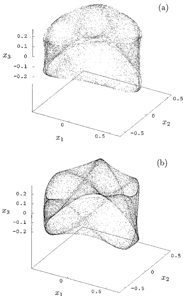
Fig. 5. (a) Projection into x_1 - x_2 - x_3 space of the period 13 237 EE orbit of Fig. 1(a) with the frequency q_x perturbed by \Delta q_x = 0.007 (see (18); 50 000 points are plotted); (b) the same initial conditions as in (a), but with \Delta q_x = 0.009585 (80 000 points are plotted). This orbit diverges after 82 197 iterations (this value depends on the machine).
