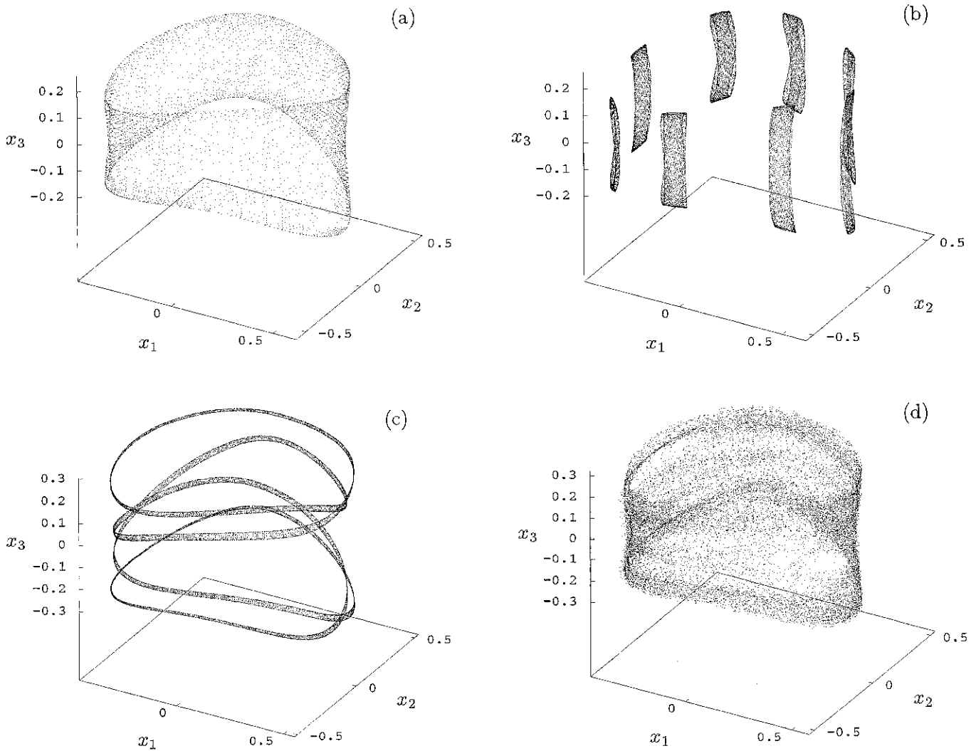
Fig. 1. Projection of different orbits into x_1 - x_2 - x_3 space, with 50 000 points plotted for (b)–(d): (a) Period 13 327 EE orbit; (b) initial conditions as in (a), with q_x disturbed by -0.001 ; (c) initial conditions of the period 16 127a orbit, with x_1 disturbed by 0.025 ; (d) orbit with the initial condition as in (c), but x_1 disturbed now by 0.005 .
