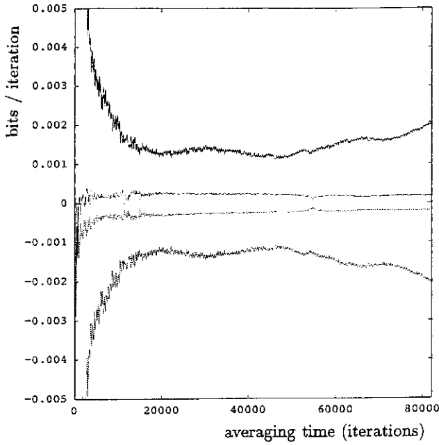
Fig. 7. Estimates of the four Lyapunov exponents \Lambda_i , using the algorithm described in the Appendix (cf. (A6), evolution time-step is 1, plotted is every 100th average). The initial conditions of the period 13 237 EE orbit are used with q_x perturbed by \Delta q_x = 0.009585 [see Figs. 5(b) and 6(b)]. Note how the slow outward diffusion of the orbits yield a maximum Lyapunov exponent which tends to grow on the average after 50 000 iterations.
