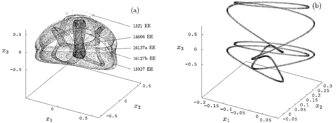
Fig. 2. Projection of different periodic EE orbits into x_1 - x_2 - x_3 space: (a) Period 1521, period 13327, period 14606, period 16127a, and the period 16127b orbit; and (b) the period 1221 orbit, whose points are lying on a curve.
