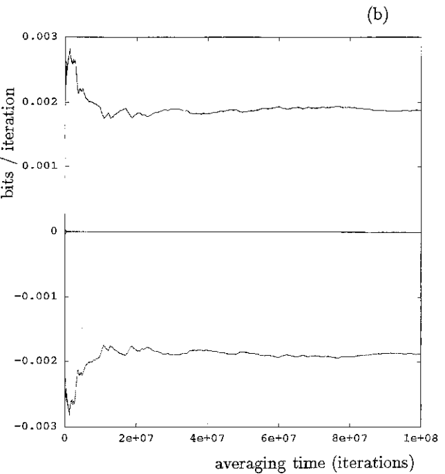
Fig. 8. The chain of eight small tori of Fig. 1b, when perturbed further by moving the initial conditions slightly outwards, yields an orbit which tends to “fill out” the region between them [see also Fig. 3(b)]; (a) the chaotic properties of this orbit are indicated by its correlation dimension (for 20 000 points (dotted) and 60 000 (solid)), which is seen to have a plateau near D_2 \simeq 2.4 at small radii; and (b) the largest Lyapunov exponent \Lambda_{max} , which approaches the value 1.9 \times 10^{-3} after N = 10^8 iterations (two exponents are almost zero).
