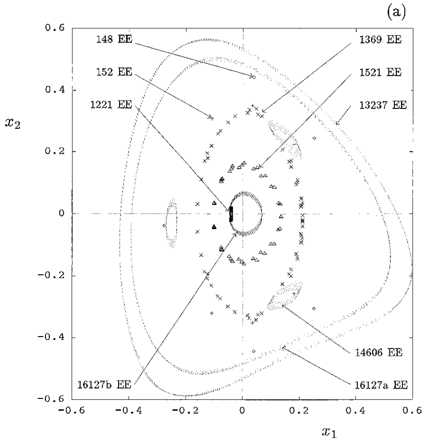
Fig. 3. (a) Different periodic EE orbits whose “cross-section” is plotted in the x_1 - x_2 plane, with |x_3| \leq 0.04 ( x_4 arbitrary); (b) same “cross-section” as in (a) for the two perturbations of the period 13237 orbit shown in Fig. 1(b) and described in Fig. 8.
