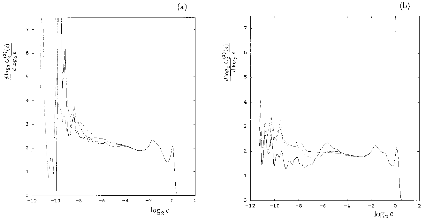
Fig. 6. Correlation dimension estimates: Slope plots [see Appendix, (A3)] are shown, calculated by using the first 10 000 (solid), 20 000 (dashed), and 30 000 (short dashes) points in each of the following cases: (a) with \Delta q_x = 0.007 [see Fig. 5(a)]; (b) with \Delta q_x = 0.009585 [see Fig. 5(b)].
