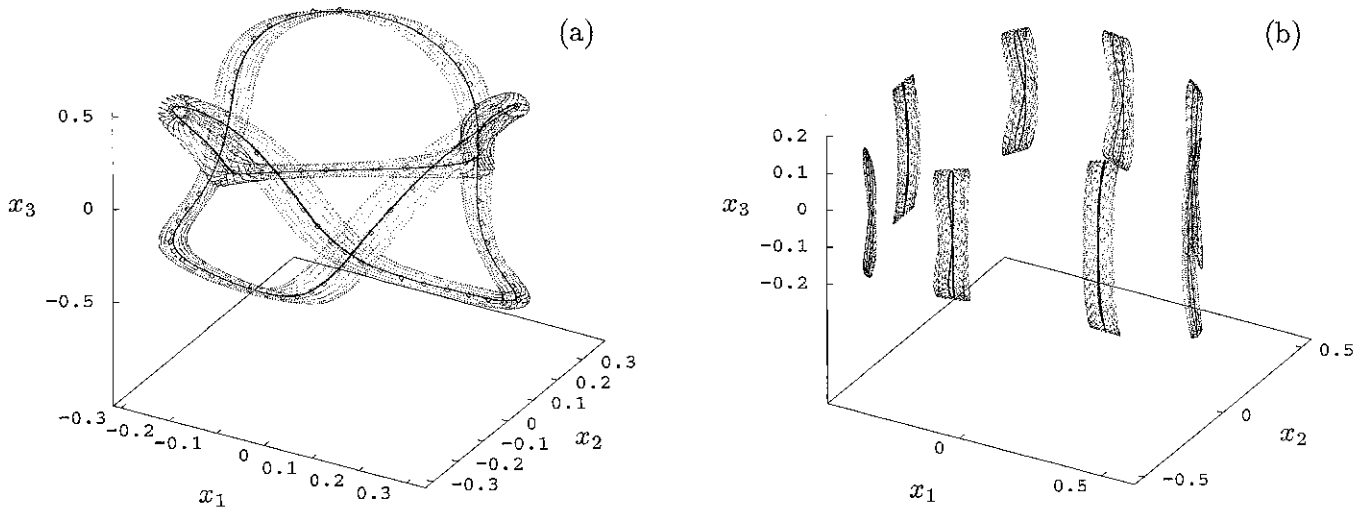
Fig. 4. Projection into x_1 - x_2 - x_3 space: (a) The period 14 606 EE orbit, together with three orbits starting near the center of the tube. Two of these orbits form a single-loop invariant curve, each, while the third one (marked with \diamond ) is periodic with period 113; (b) a perturbation [ \Delta q_w = -0.001 ; see Fig. 1(b)] of the period 13 237 orbit yielding a chain of eight small tori, in the "interior" of which one finds a set of disconnected multi-loop curves.
